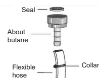
Flexible hose
