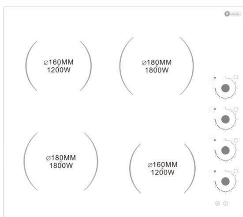
HTR4MV60V2
