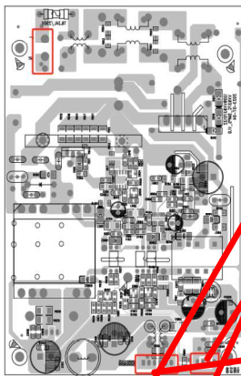
Power board PCBA
